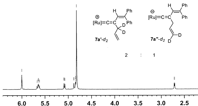
Figure 1. Part of the 1 H NMR spectrum of the mixture containing 7a'-d_2 and 7a''-d_2 obtained from 99% deuterated 5a-d 2 at 60 °C.
